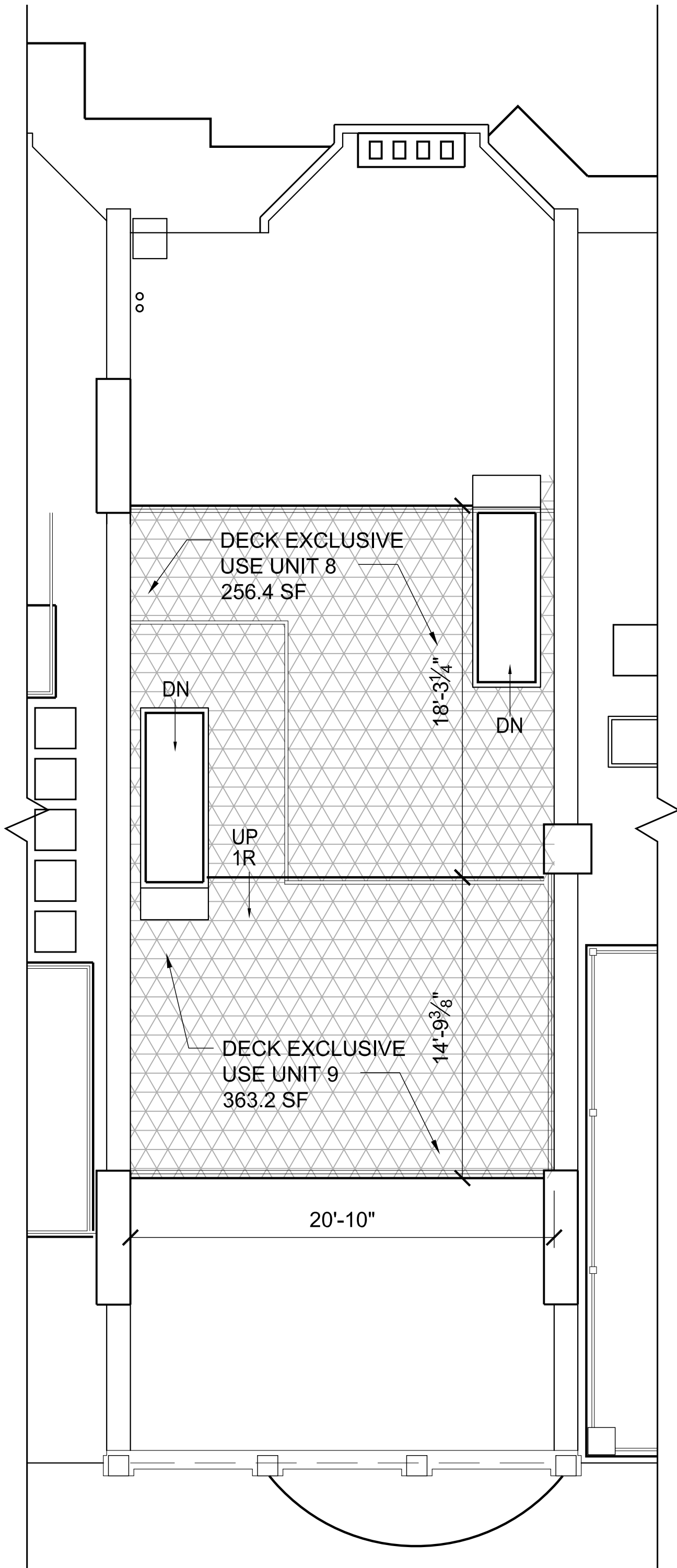
6 ROOF PLAN 1/8"=1'-0"
